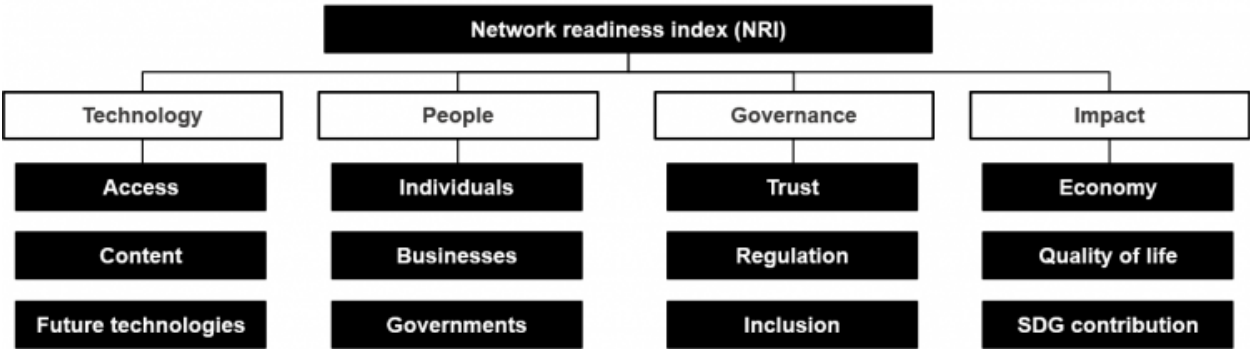
Figure 3. The NRI* 2019 model [6].
